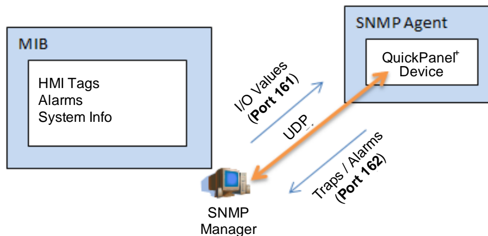
QuickPanel+ as SNMP Agent
