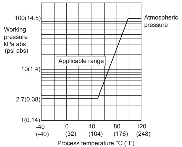
Figure 2. Working Pressure and Process Temperature
