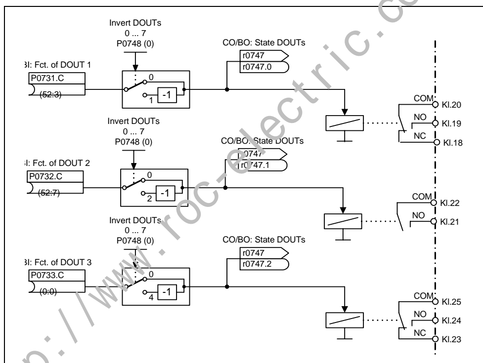
Fig. 2-30 Digital outputs
